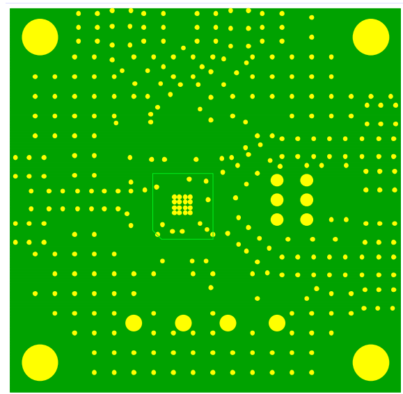
Figure 55. Evaluation Board Ground Plane, Internal Layer 1
