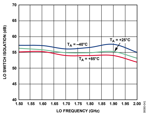
Figure 33. LO Switch Isolation vs. LO Frequency
