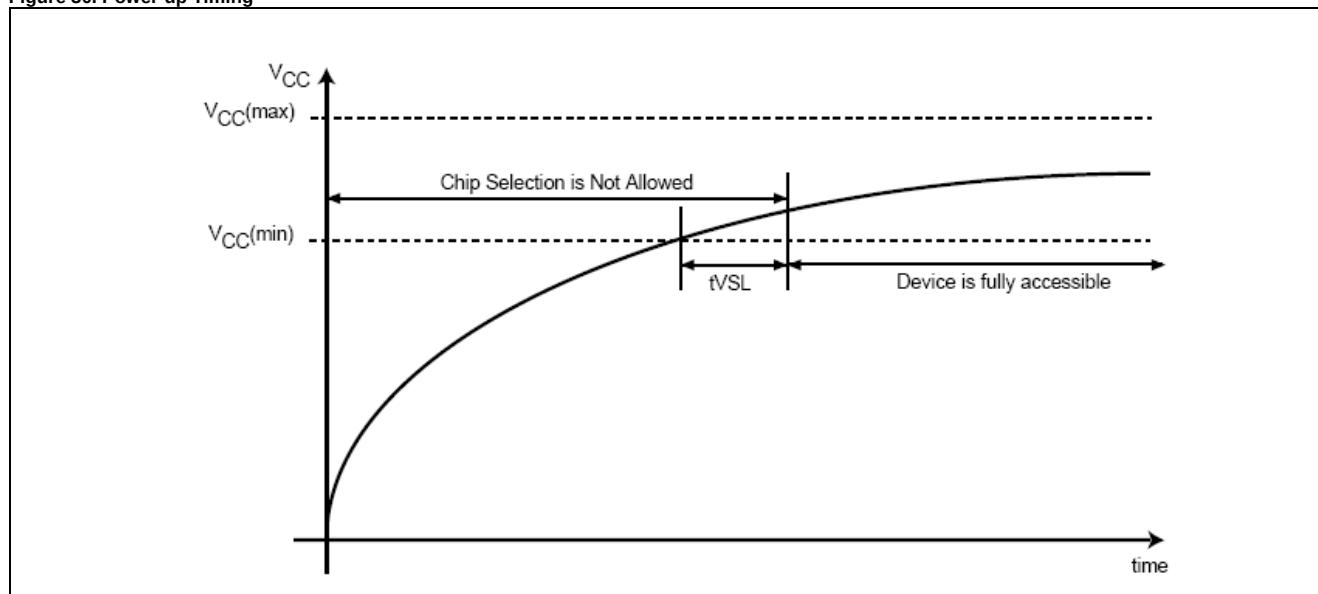
Figure 30. Power-up Timing
