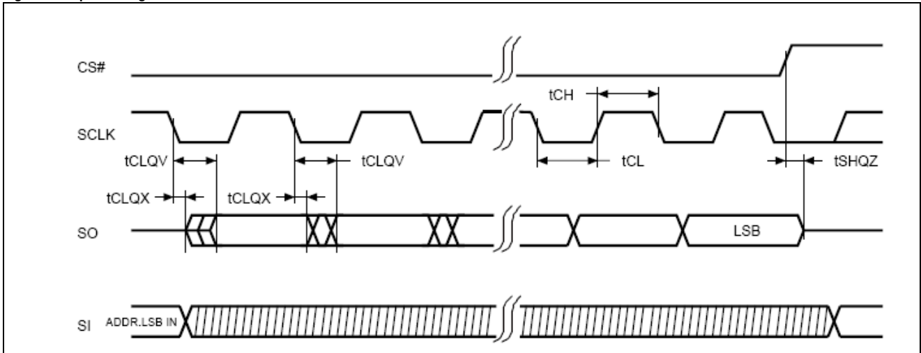
Figure8. Output Timing
