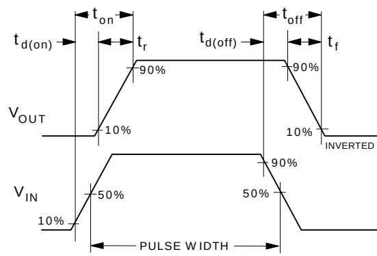
Figure 12. Switching Waveforms
