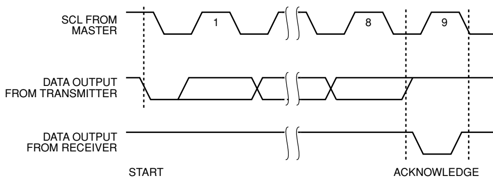
Figure 4. Acknowledge Timing
