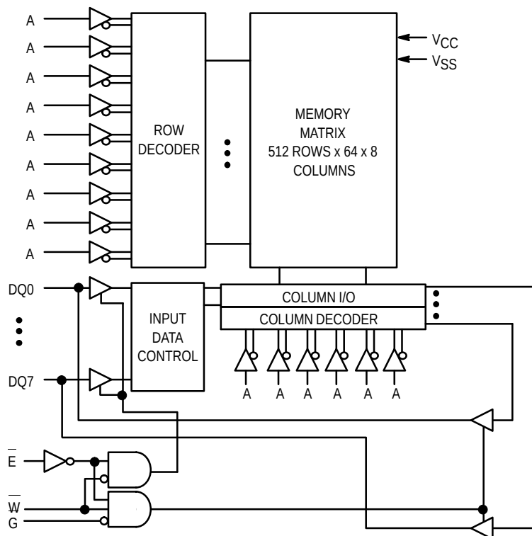
BLOCK DIAGRAM
