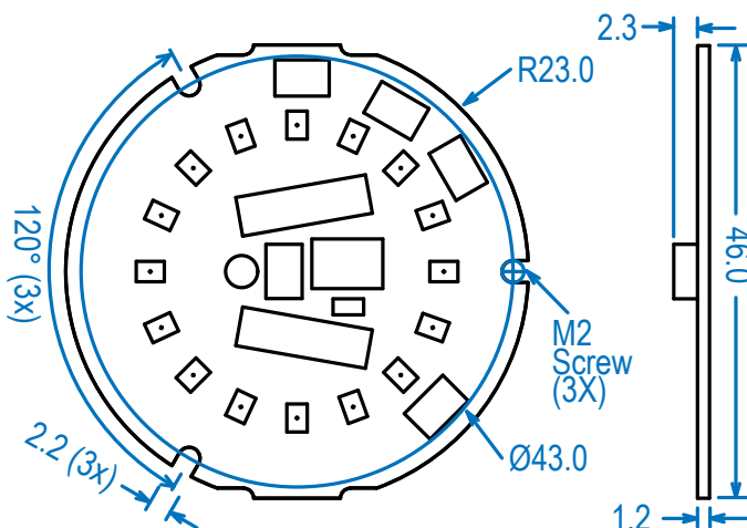
"Warm Dimming" 46mm 120V AC Round LED Module 9W
