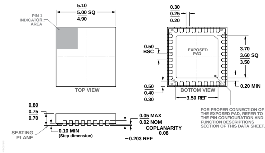
Figure 35. 32-Lead Lead Frame Chip Scale Package [LFCSP_SS] 5 mm × 5 mm Body with Side Solderable Leads (CS-32-3) Dimensions shown in millimeters
