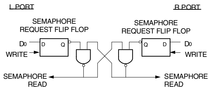
Figure 4. IDT7034 Semaphore Logic
