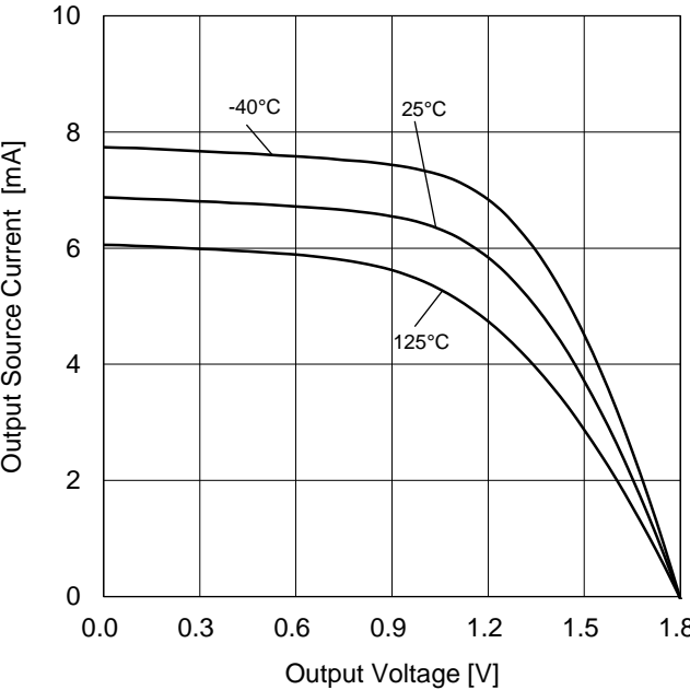
Figure 9. Output Source Current vs Output Voltage (VDD=1.8V)
