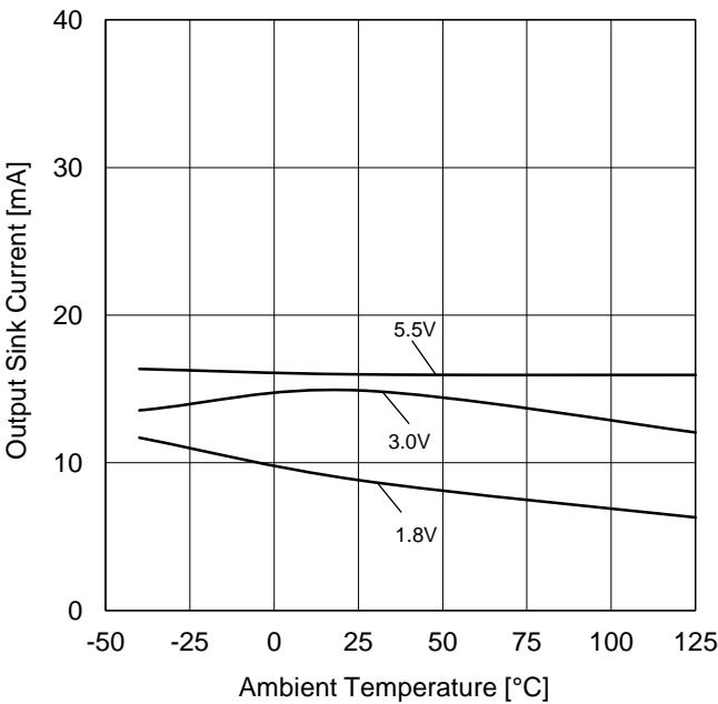
Figure 16. Output Sink Current vs Ambient Temperature (OUT=VSS+0.4V)
