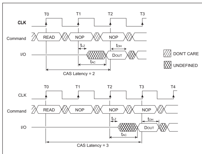
FIGURE 4 – CAS LATENCY
