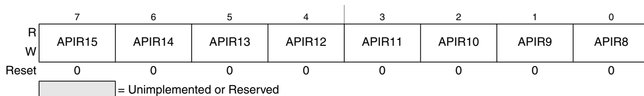
Figure 23-6. Autonomous Periodical Interrupt Rate High Register (VREGAPIRH)
