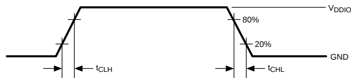
Figure 10. Deserializer LVCMOS Transition Times
