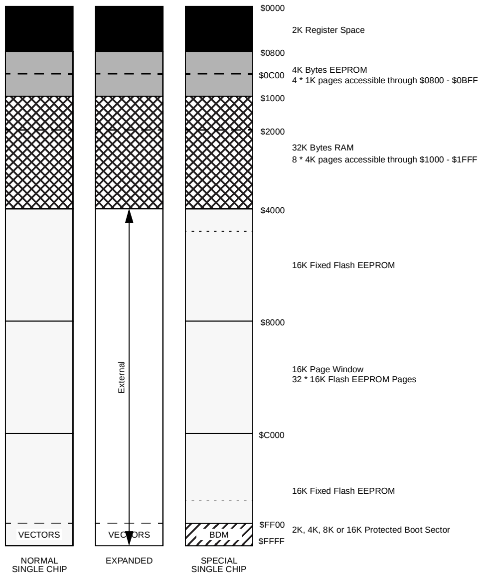
Figure 4. MC9S12XD-Family Memory Map 1
