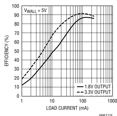
Efficiency (Wall Powered)
