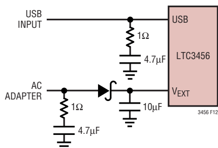
Figure 12. Bypassing USB and AC Wall Adapter Inputs
