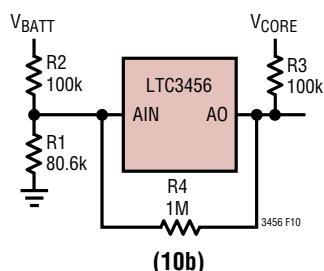
Figure 10. Low-Battery Detector (10a) and Low-Battery Detector with Hysteresis (10b)
