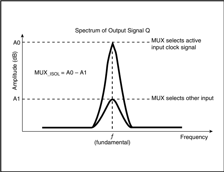
MUX Isolation
