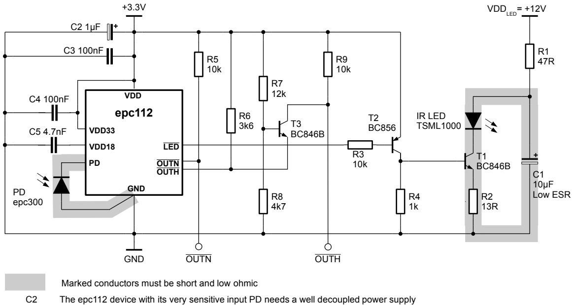
Figure 11: High speed detection rate light barrier application with minimal part count
