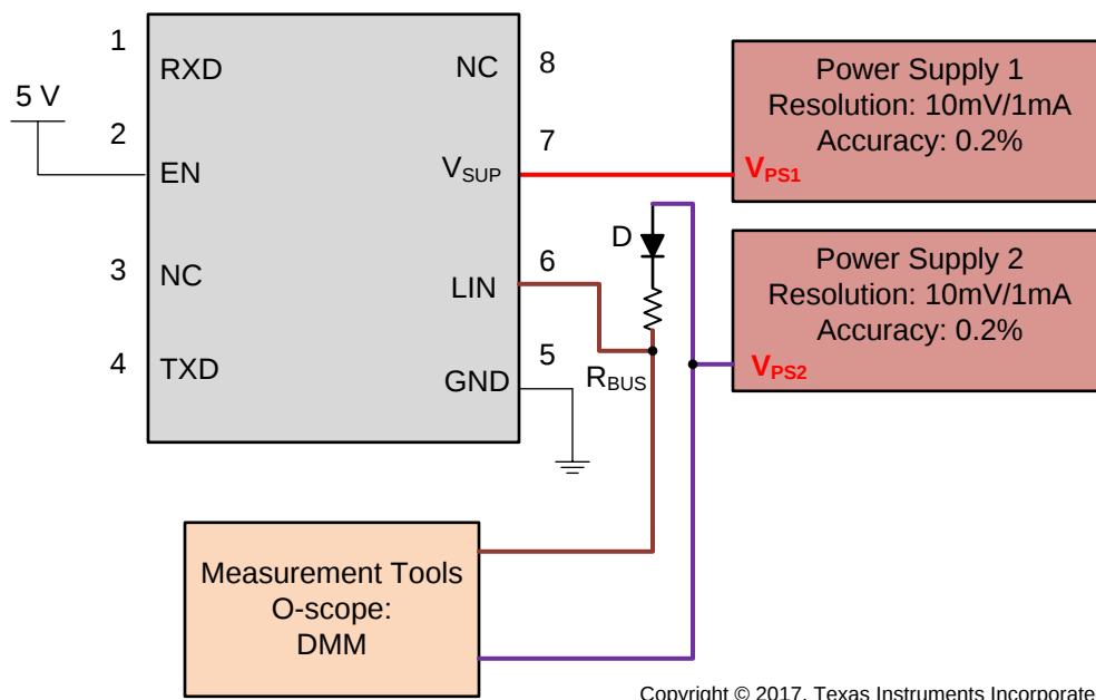
Figure 12. V_{SUP\_NON\_OP} Param 1154/56
