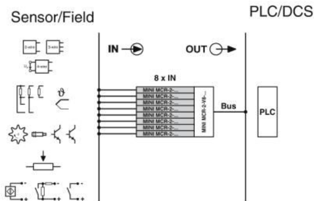
Block diagram
