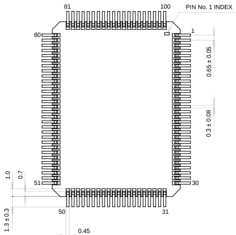
PACKAGE STRUCTURE
