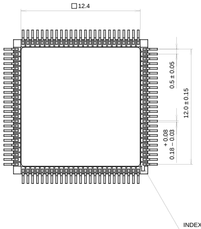
PACKAGE STRUCTURE
