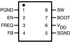
Figure 2. Top View
