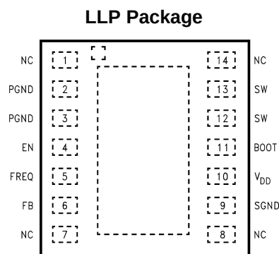
Figure 1. Top View
