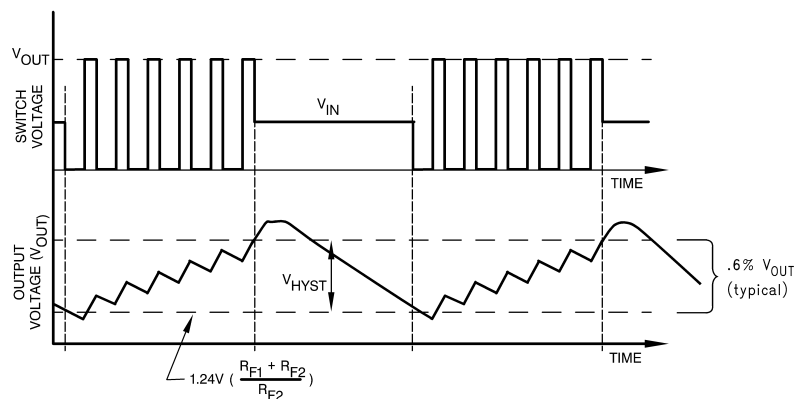
Figure 4. Typical Step-Up Regulator Waveforms
