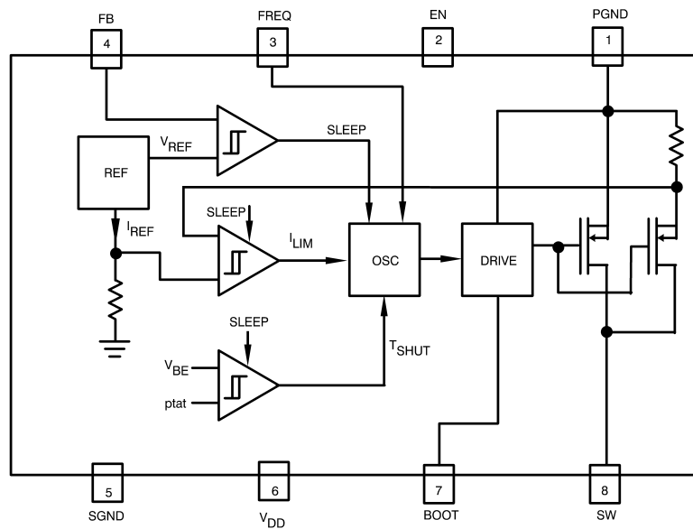
Figure 3. Functional Diagram
