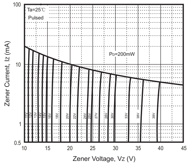
Fig.2 - Zener Characteristics (11V to 39V)
