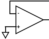
FIGURE 66. PREVENTING OSCILLATIONS IN UNUSED CHANNELS
