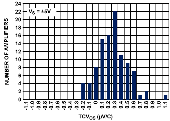
FIGURE 16. ISL28208 TDFN TCV OS vs NUMBER OF AMPLIFIERS, V_S = \pm 5V
