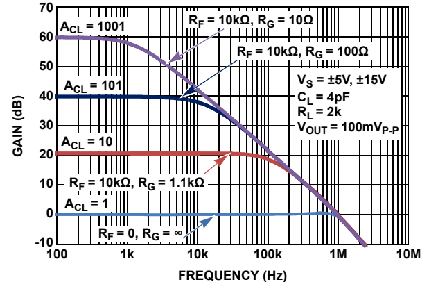
FIGURE 44. FREQUENCY RESPONSE vs CLOSED LOOP GAIN
