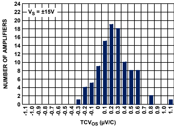
FIGURE 15. ISL28208 TDFN TCV OS vs NUMBER OF AMPLIFIERS, V_S = \pm 15V
