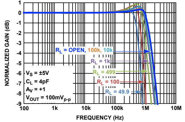
FIGURE 46. GAIN vs FREQUENCY vs R_L , V_S = \pm 15V
