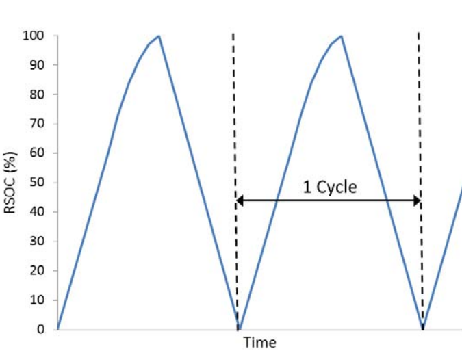
Figure 21. Discharge/Charge cycle
