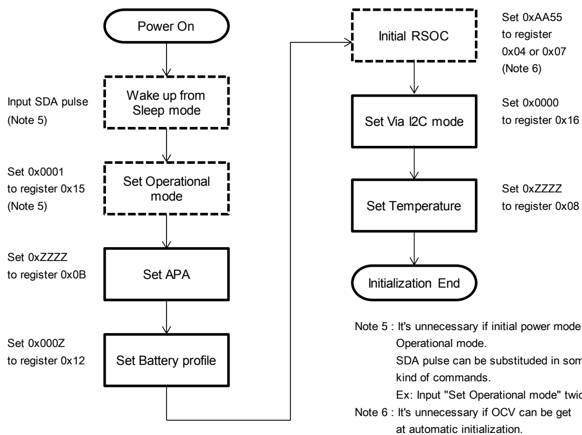
Figure 18. Starting flow at I 2 C mode
