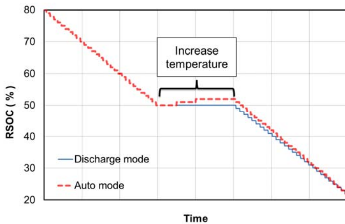
Figure 10. Discharge Mode
