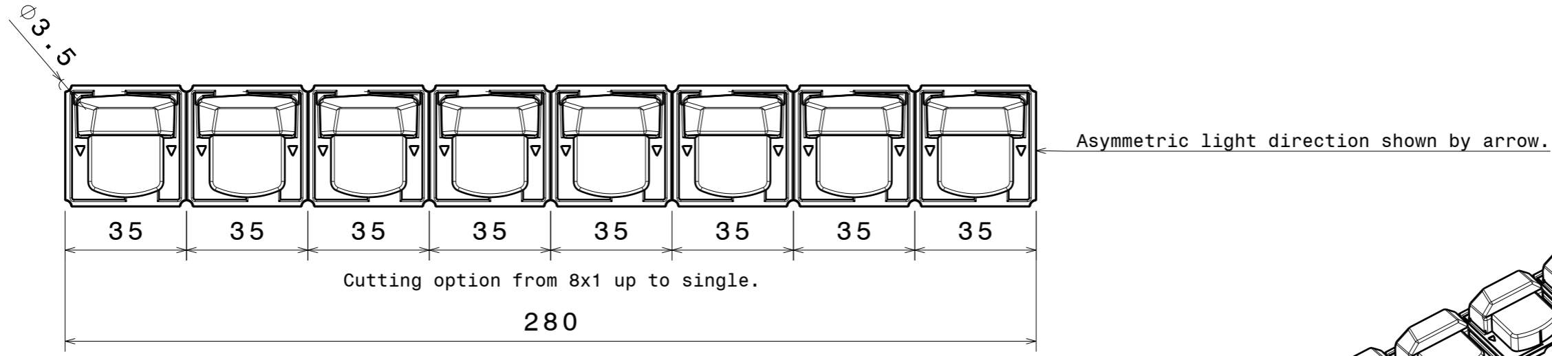
Top view
