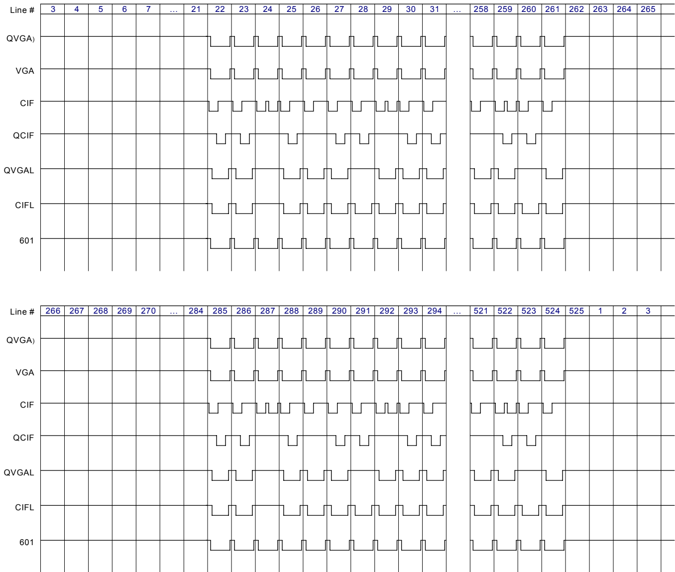
Input Video Signal vs Output Data Relationship (NTSC)
