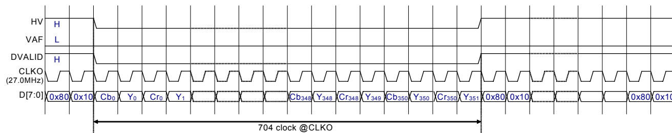
Timing Chart (Camera I/F)
