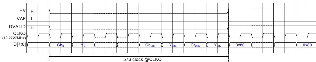
Timing Chart (Camera I/F) Rotated CIF (NTSC) Register Set: VLF = 1'b0, OFORM[2:0] = 3'b101, OIF[1:0] = 2'b00
