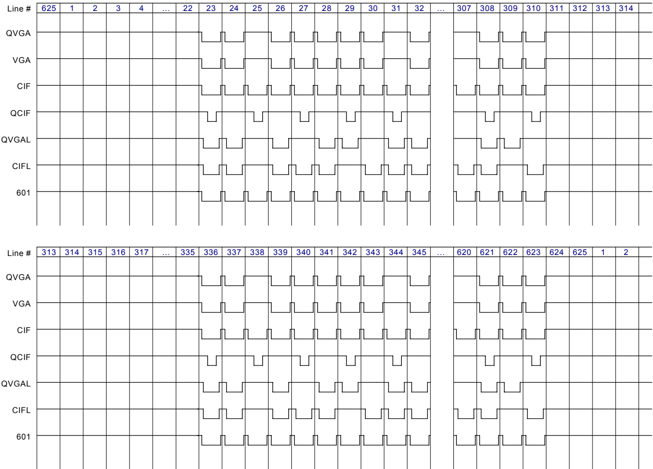
Input Video Signal vs Output Data Relationship (PAL)
