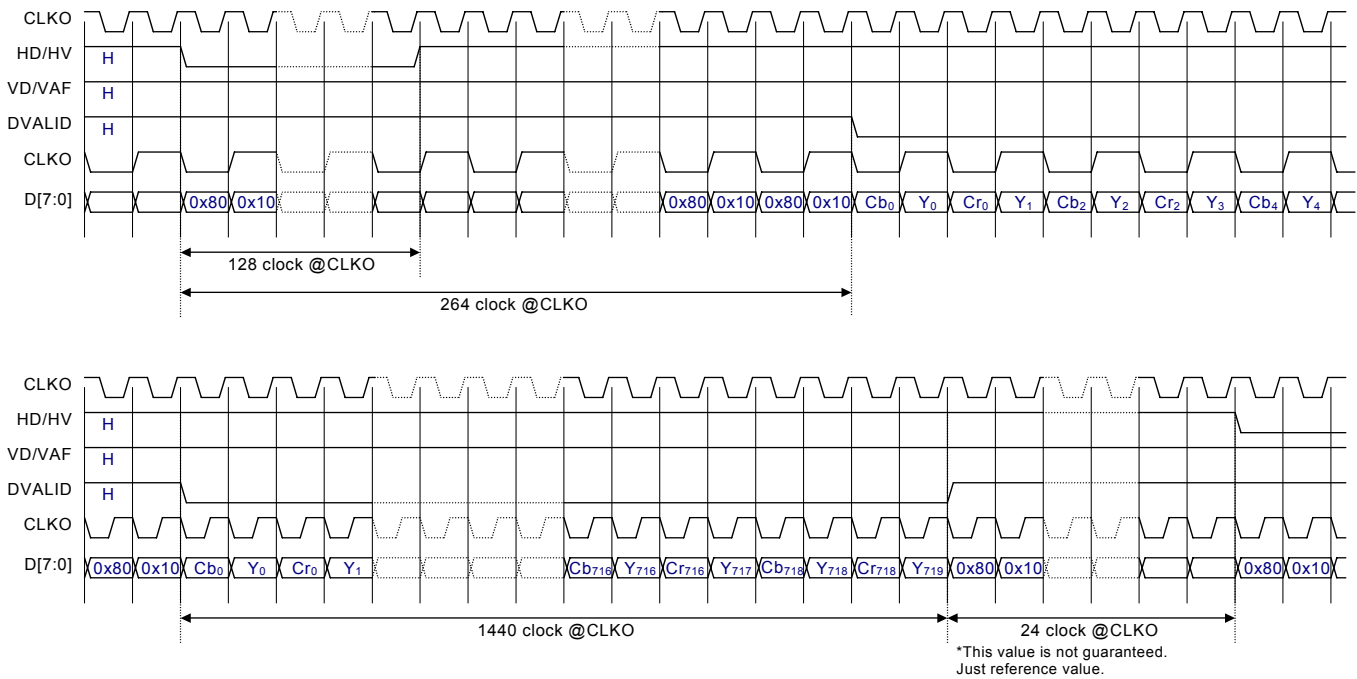
Timing Chart 601output (PAL) 2'b10
