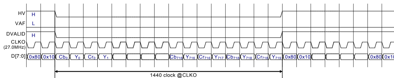
Timing Chart (Camera I/F) 601Output (NTSC) Register Set: VLF = 1'b0, OFORM[2:0] = 3'b110, OIF[1:0] = 2'b00
