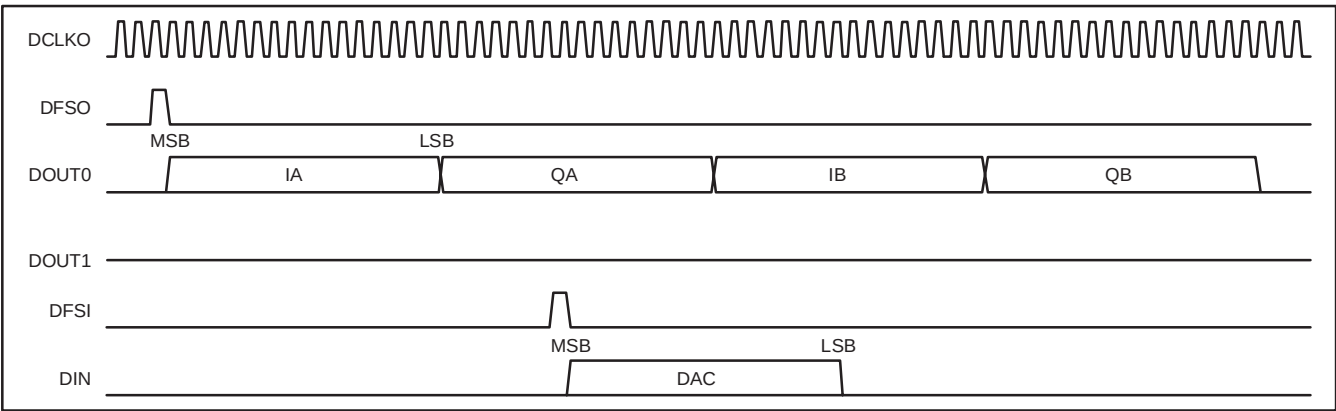
Figure 12. Data Interface Timing for MODE = 0
