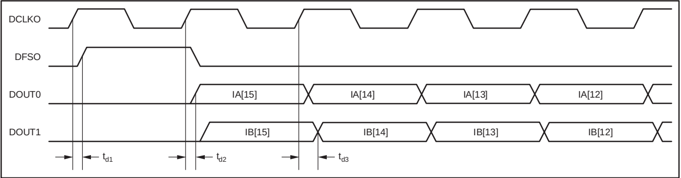
Figure 1. Data Interface Timing 1
