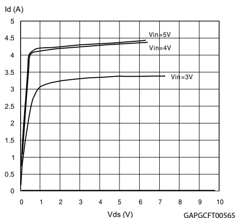
Figure 24. Output characteristics
