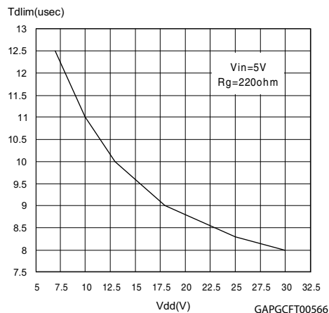
Figure 25. Step response current limit
