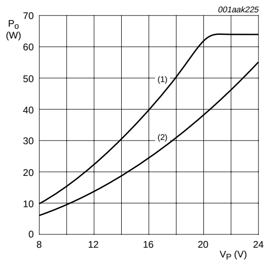
THD = 0.5 %. R_{DSon} = 0.19 \, \Omega (at T_j = 100 \, ^\circ\text{C} ), R_s = 0.05 \, \Omega , t_{w(min)} = 190 \, \text{ns} and I_{O(ocp)} = 8 \, \text{A} (minimum). (1) R_L = 2 \, \Omega . (2) R_L = 4 \, \Omega .
