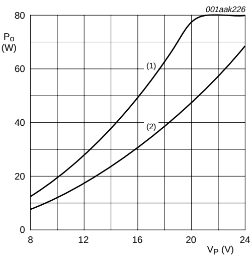
THD = 10 %. R_{DSon} = 0.19 \, \Omega (at T_j = 100 \, ^\circ\text{C} ), R_s = 0.05 \, \Omega , t_{w(min)} = 190 \, \text{ns} and I_{O(ocp)} = 8 \, \text{A} (minimum). (1) R_L = 2 \, \Omega . (2) R_L = 4 \, \Omega .
