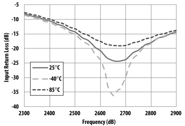
Figure 23. IRL vs Frequency and Temperature
