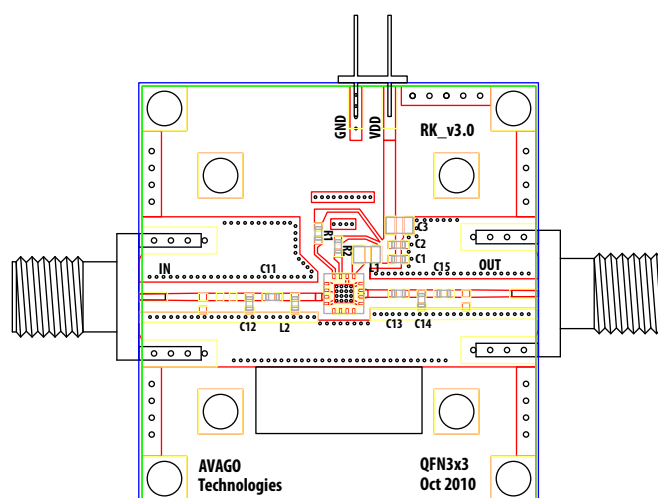
Figure 47. Demoboard
