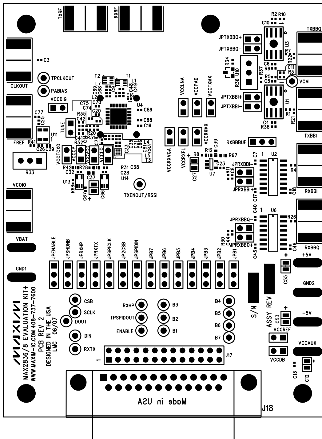
Figure 4. MAX2838 EV Kit PCB Layout—Top Silkscreen
