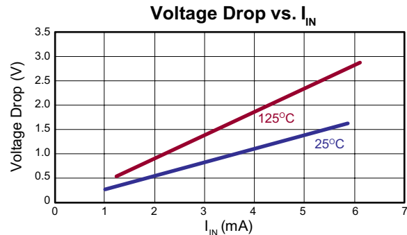
Fig. 1. Maximum Voltage Drop vs. Input Current
