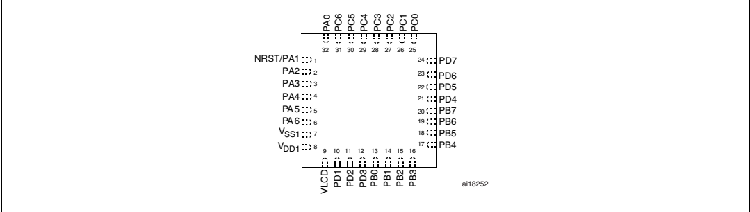
Figure 8. STM8L152Kx 32-pin package pinout (with LCD)
