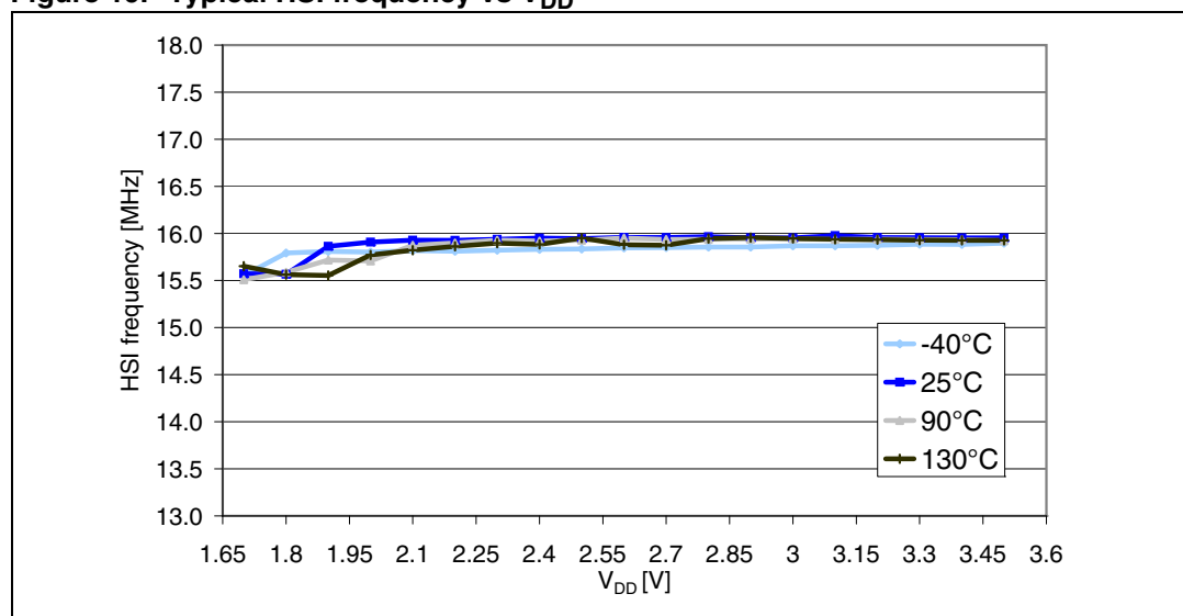
Figure 19. Typical HSI frequency vs V_{DD}
