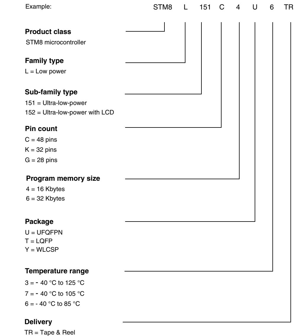
Figure 54. Medium density STM8L15x ordering information scheme
