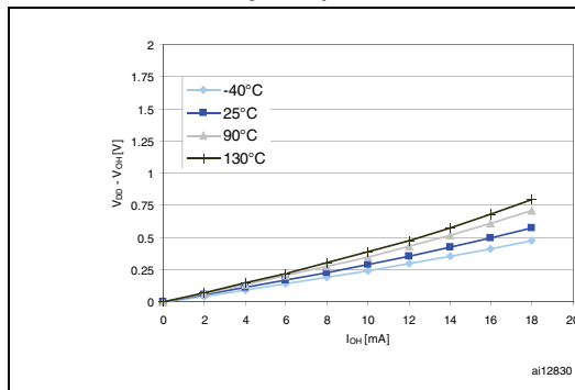
Figure 29. Typ. V_{DD} - V_{OH} @ V_{DD} = 3.0\text{ V} (high sink ports)
