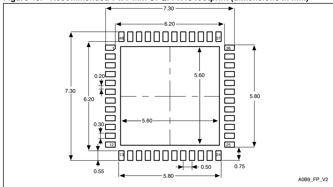
Figure 46. Recommended 7 x 7 mm UFQFPN48 footprint (dimensions in mm)
