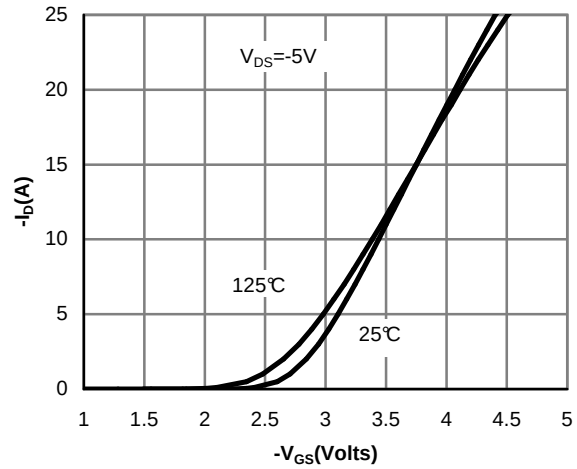
Figure 2: Transfer Characteristics 850
