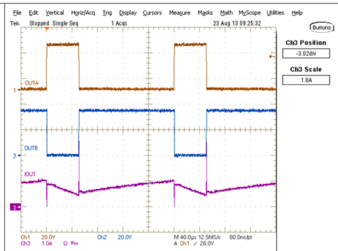
Figure 13. Reverse Drive, Fast Decay
