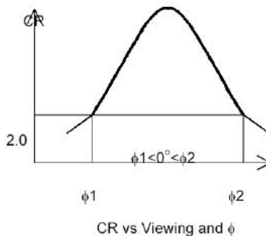
Note 2. Definition of Viewing angle \phi 1 and \phi 2
