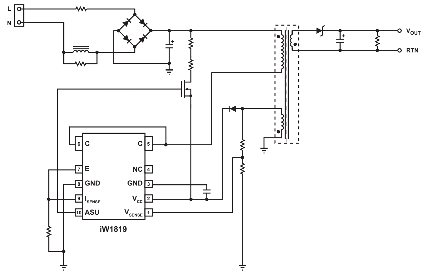
Figure 3.1 : iW1819 Typical Application Circuit
