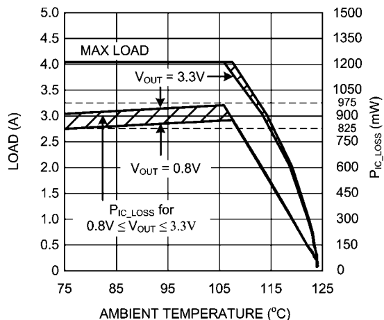
Current Derating V_{IN} = 5V , \theta_{JA} = 20^{\circ}C/W
