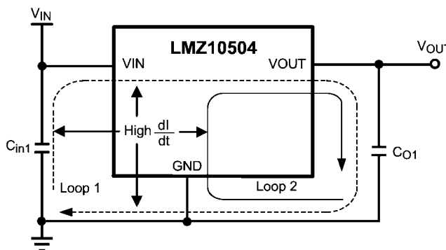
FIGURE 1. High Current Loops
