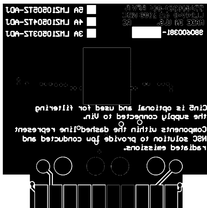
FIGURE 9. Bottom Copper
