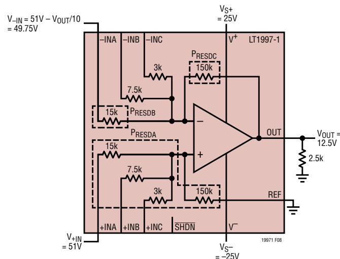
Figure 8. Power Dissipation Example
