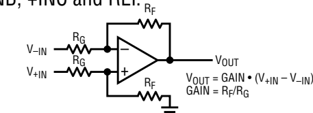
DIFFERENCE AMPLIFIER CONFIGURATION
