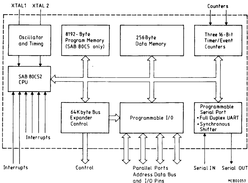
Figure 1 Block Diagram
