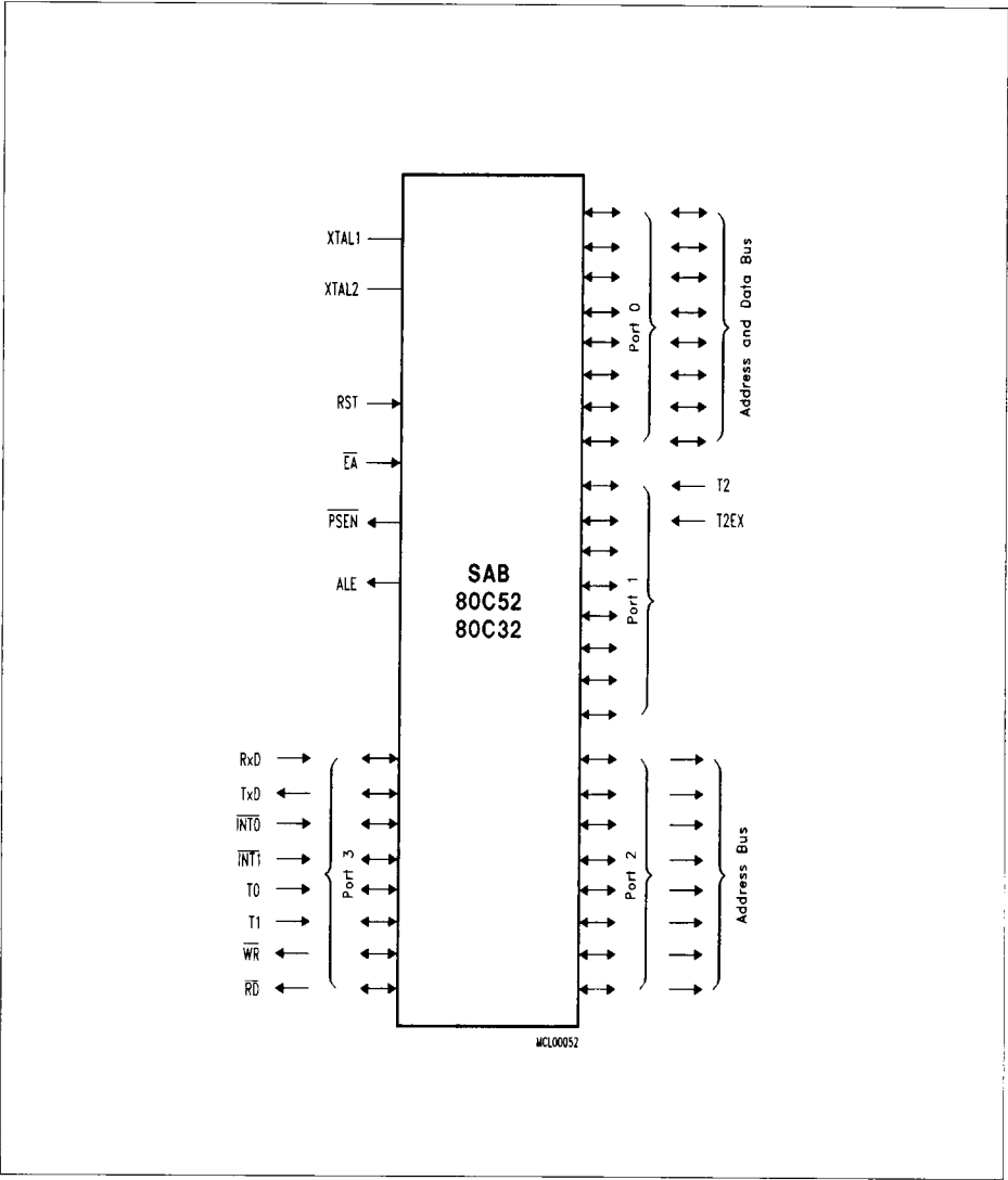
Logic Symbol
