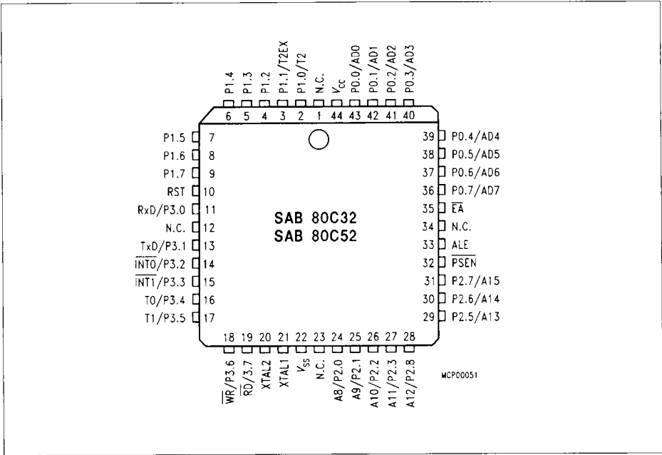
Pin Configuration (P-LCC-44)
