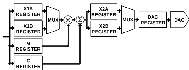
Figure 8. Data Registers Associated With Each DAC Channel
