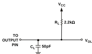
Figure 2. Load Circuit for \overline{BUSY} Timing Diagram
