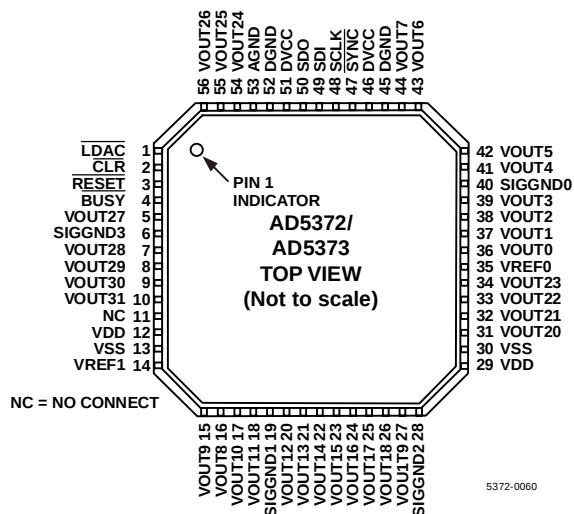
Figure 7. 56-Lead LFCSP Pin Configuration
