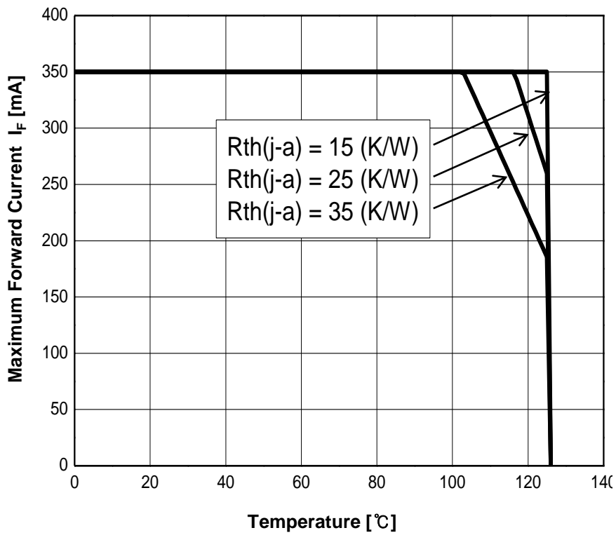
Fig 9. Maximum Forward Current vs. Temperature
