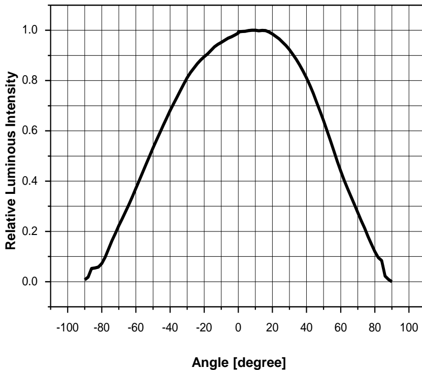
Fig 2. Viewing Angle Distribution, I_F = 250\text{mA}
