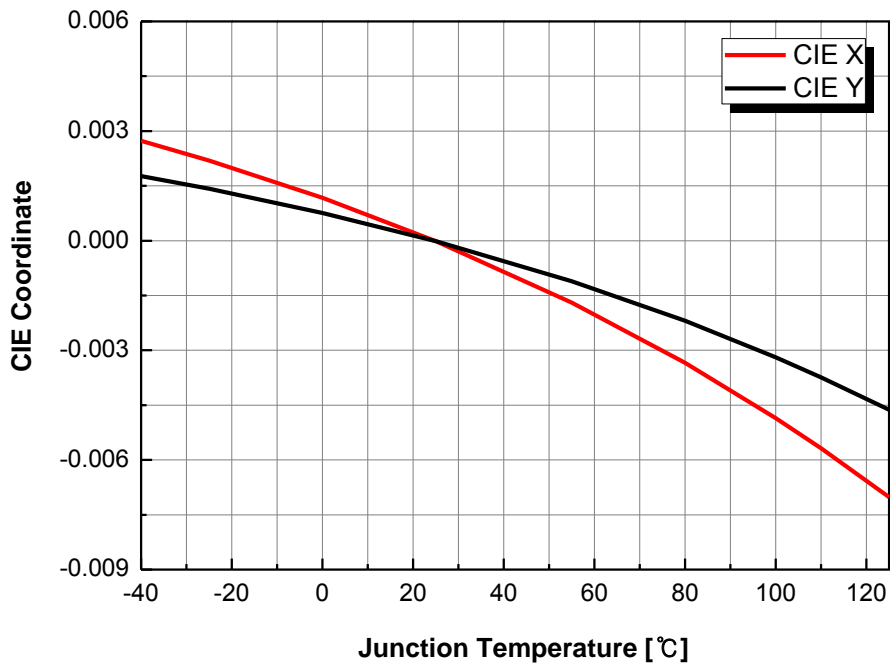
Fig 8. Chromaticity Coordinate vs. Junction Temperature, I_F = 250\text{mA}
