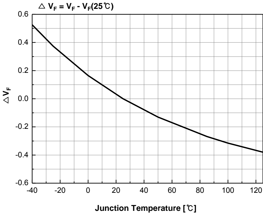
Fig 7. Junction Temperature vs. Forward Voltage Shift, I_F = 250\text{mA}
