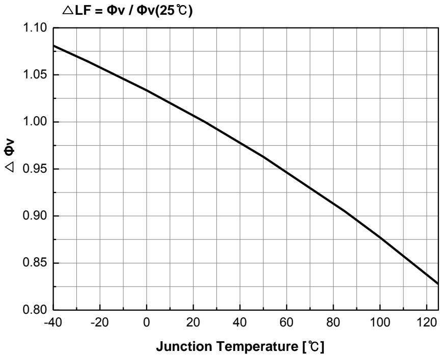
Fig 6. Relative Light Output vs. Junction Temperature, I_F = 250\text{mA}
