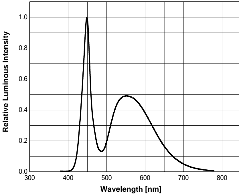
Fig 1. Color Spectrum, I_F = 250\text{mA} , T_j = 25^\circ\text{C} , RH30%
