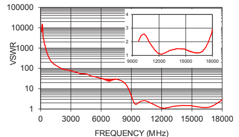
HFCN-9700+ VSWR
