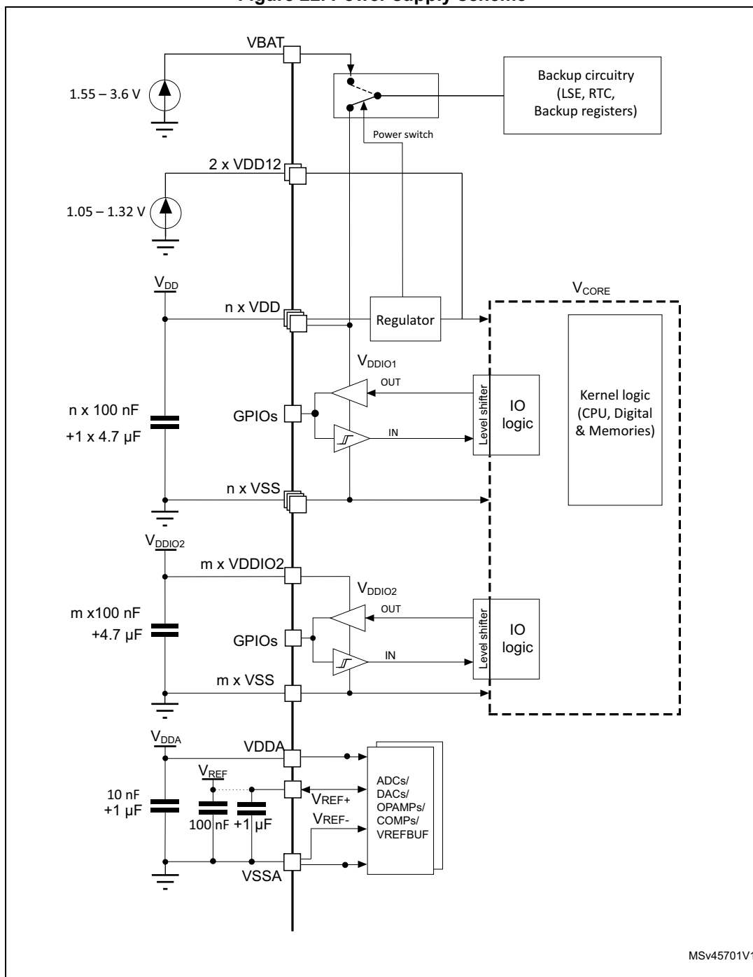
Figure 22. Power supply scheme
