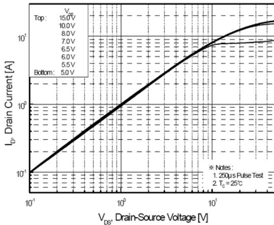
Fig. 1 On-State Characteristics
