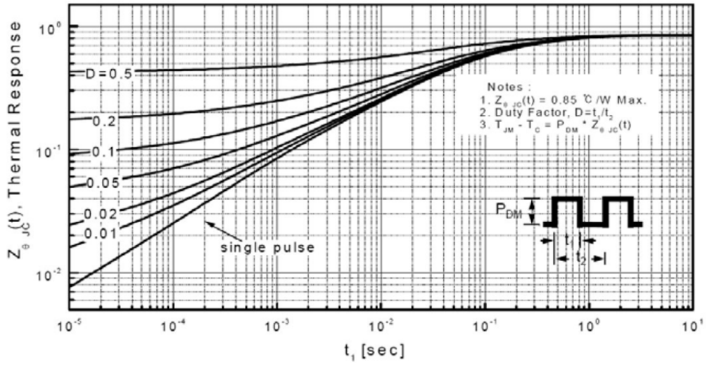
Fig. 9 Transient Thermal Response Curve(TO-220AB)
