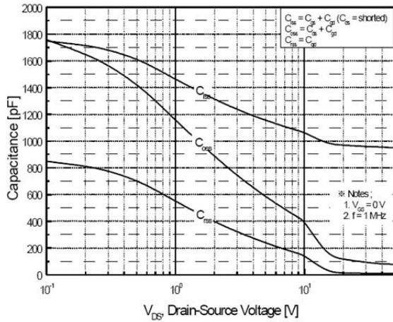
Fig. 5 Capacitance Characteristics
