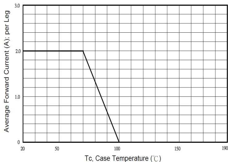
Typical Forward Current Derating Curve
