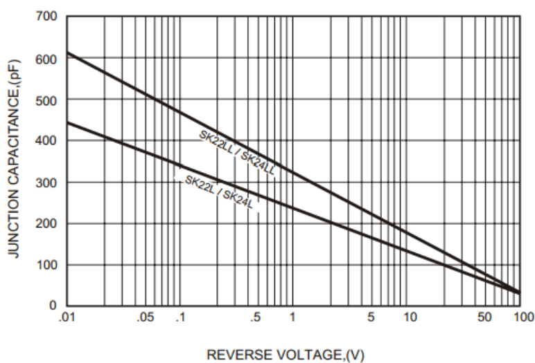
FIG.3-TYPICAL JUNCTION CAPACITANCE
