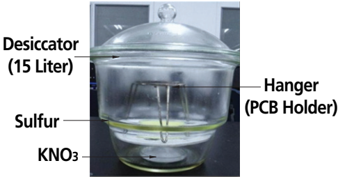
[ Test Equipment ]
