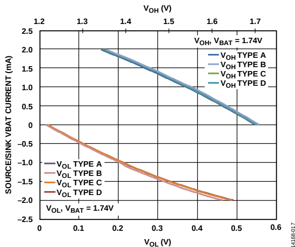
Figure 17. Output Single Drive Strength Characteristics ( V_{BAT} = 1.74\text{ V} )
