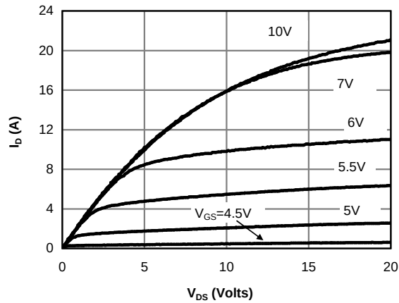
Figure 1: On-Region Characteristics@25°C
