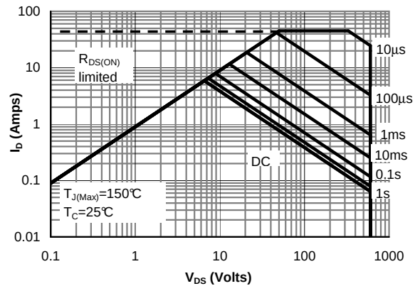
Figure 12: Maximum Forward Biased Safe Operating Area for AOTF11S60 (Note F)
