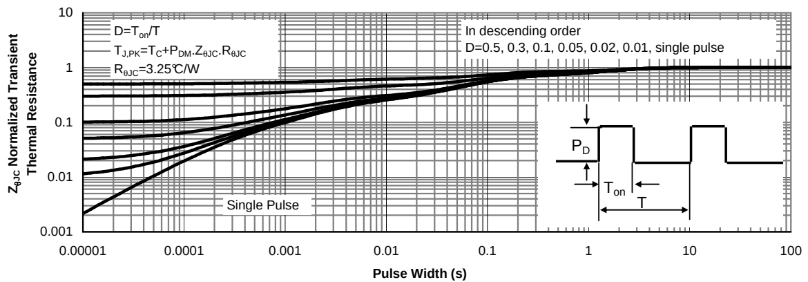
Figure 16: Normalized Maximum Transient Thermal Impedance for AOTF11S60 (Note F)
