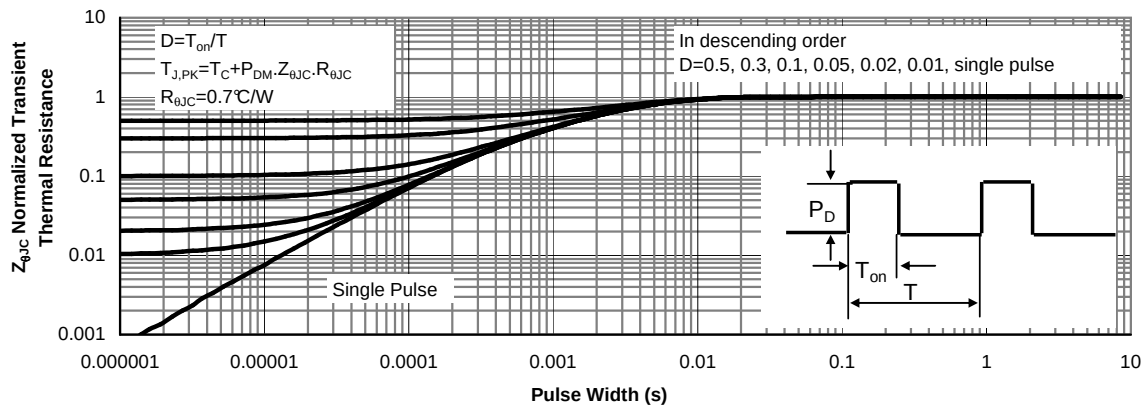
Figure 15: Normalized Maximum Transient Thermal Impedance for AOT(B)11S60 (Note F)
