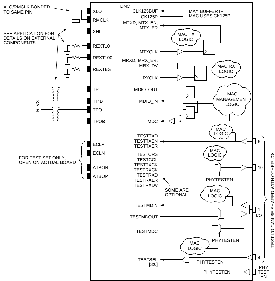
Figure 6. Typical Application (One Channel Shown)
