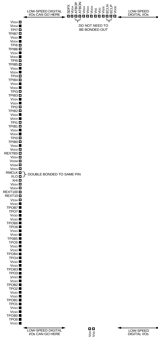
Figure 7. Pinout Assignment
