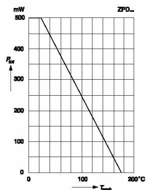
Admissible power dissipation versus ambient temperature
